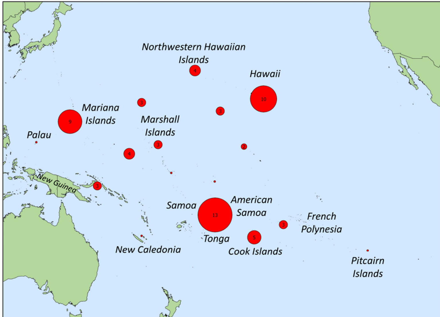
Figure 5. Clusters of Goose-beaked whale ( Z. cavirostris ) stranding events across the Pacific Islands. Number of stranding events represented by individual clusters determined by geographic distance are provided in the center of each cluster.
