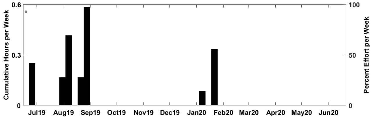
Figure 16. Weekly presence of Gervais' / True's beaked whale echolocation clicks from June 2019 to 2020 at JAX Site D. Effort markings are described in Figure 14.
