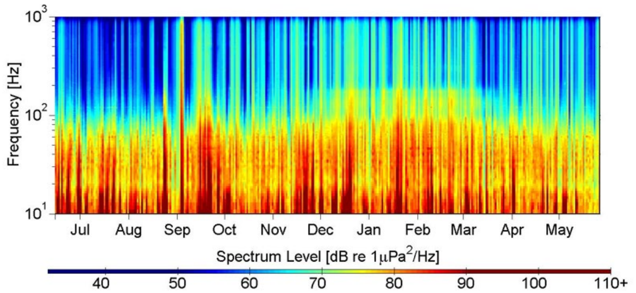
Figure 13. Long-term spectrograms using daily-averaged spectra for JAX Site D from June 2019 to 2020.
