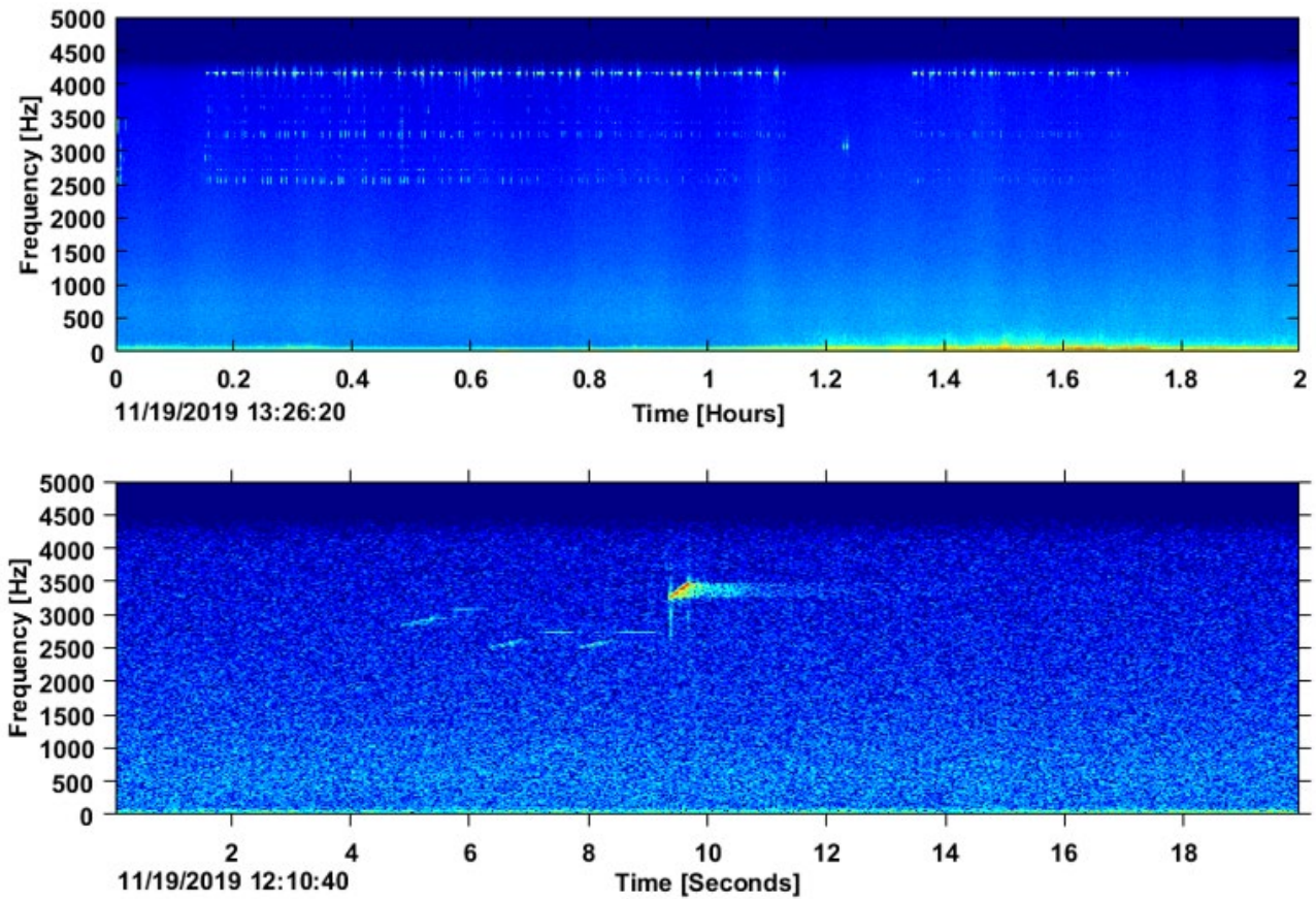
Figure 10. Mid-Frequency Active (MFA) sonar in LTSA (top) and spectrogram (bottom) recorded at JAX Site D, November 2019.
