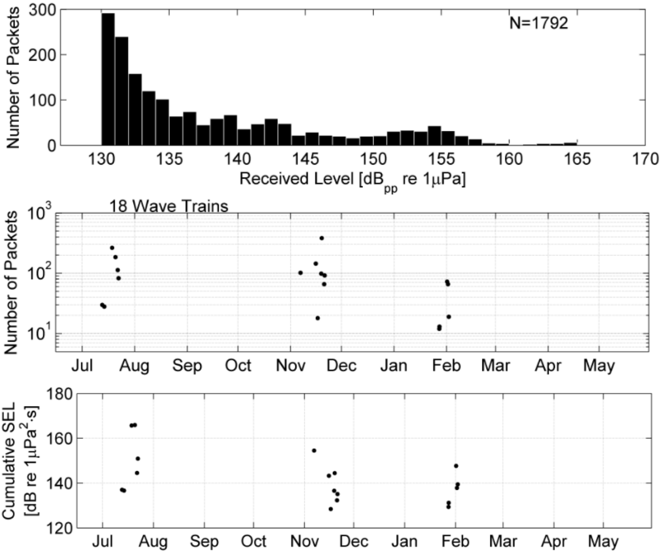
Figure 24. Top: Distribution of received levels (RL) of detected MFA packets. Center: Number of MFA packets detected in each wave train exceeding the minimum RL threshold (130 dB pp re 1 \mu\text{Pa} ). Bottom: Cumulative Sound Exposure Levels (CSEL) associated with each wave train.
