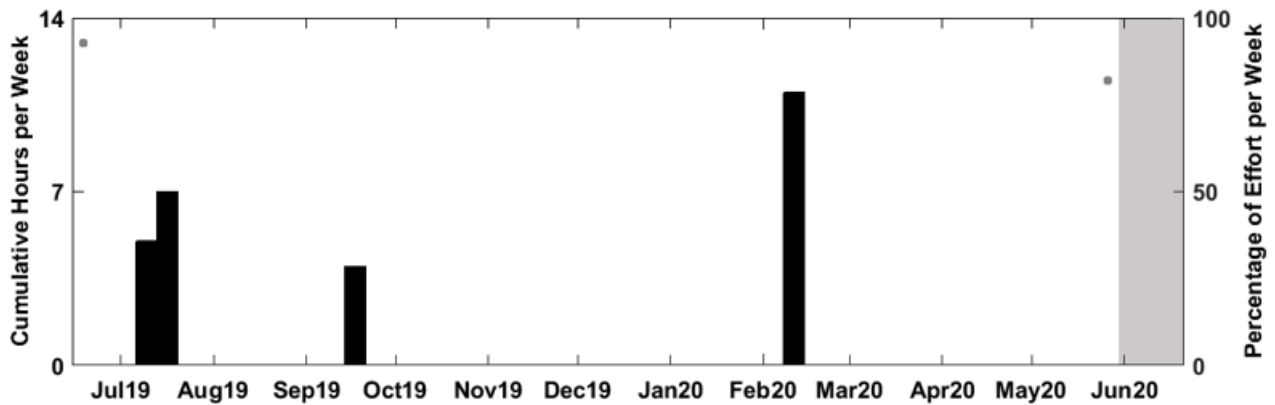
Figure 20. Weekly presence of LFA sonar from June 2019 to 2020 at JAX Site D. Effort markings are described in Figure 14.
