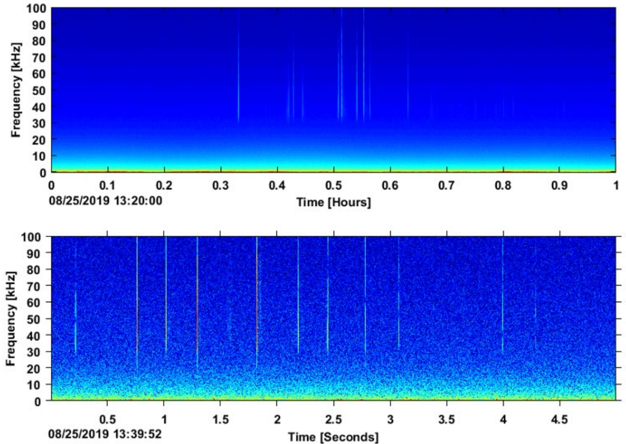
Figure 5. Gervais' beaked whale signals in LTSA (top) and spectrogram (bottom) recorded at JAX Site D, August 2019.
