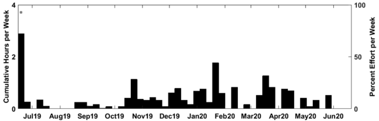
Figure 18. Weekly presence of Kogia spp. clicks from June 2019 to 2020 at JAX Site D. Effort markings are described in Figure 14.
