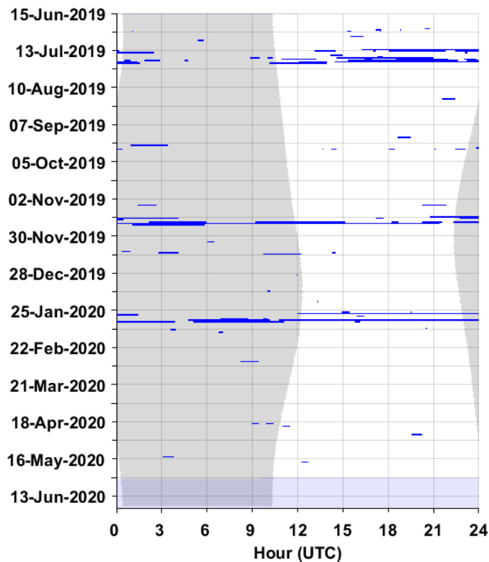
Figure 23. MFA sonar less than 5 kHz in five-minute bins from June 2019 to 2020 at JAX Site D. Effort markings are described in Figure 15.
