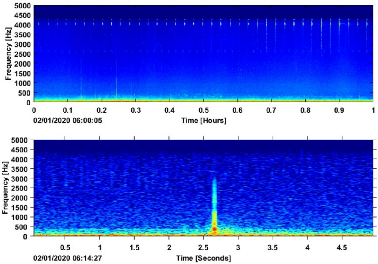
Figure 11. Explosions in LTSA (top) and spectrogram (bottom) recorded at JAX Site D, February 2020.
