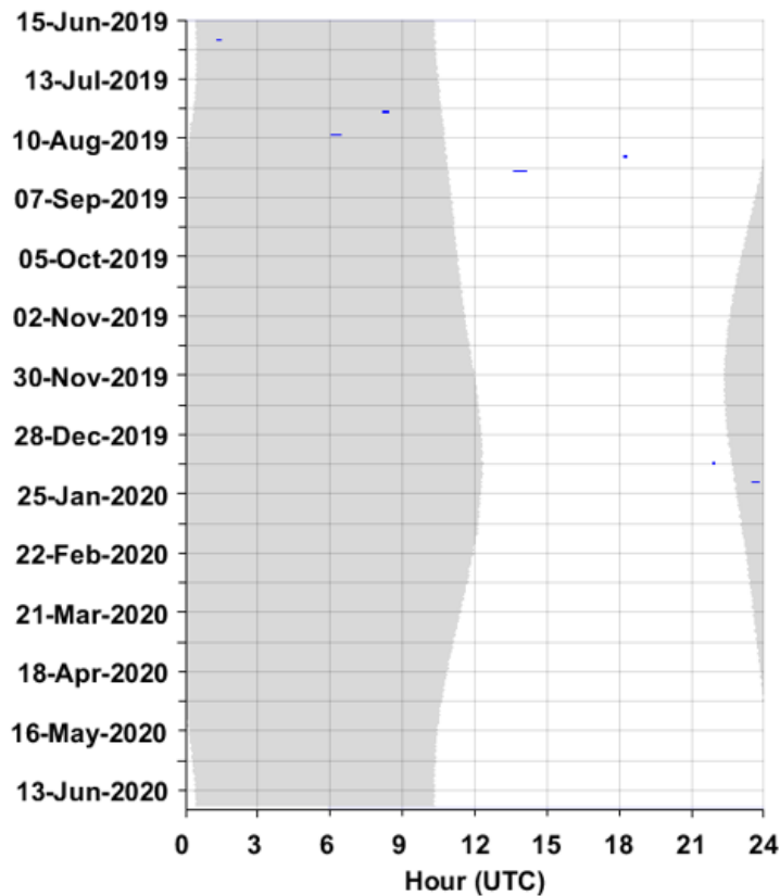
Figure 17. Gervais' / True's beaked whale echolocation clicks in five-minute bins from June 2019 to 2020 at JAX Site D. Effort markings are described in Figure 15.
