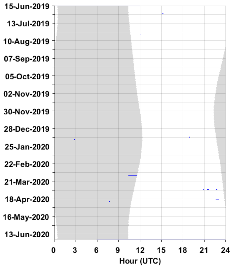
Figure 15. Cuvier’s beaked whale echolocation clicks in five-minute bins from June 2019 to 2020 at JAX Site D. Gray vertical shading denotes nighttime.
