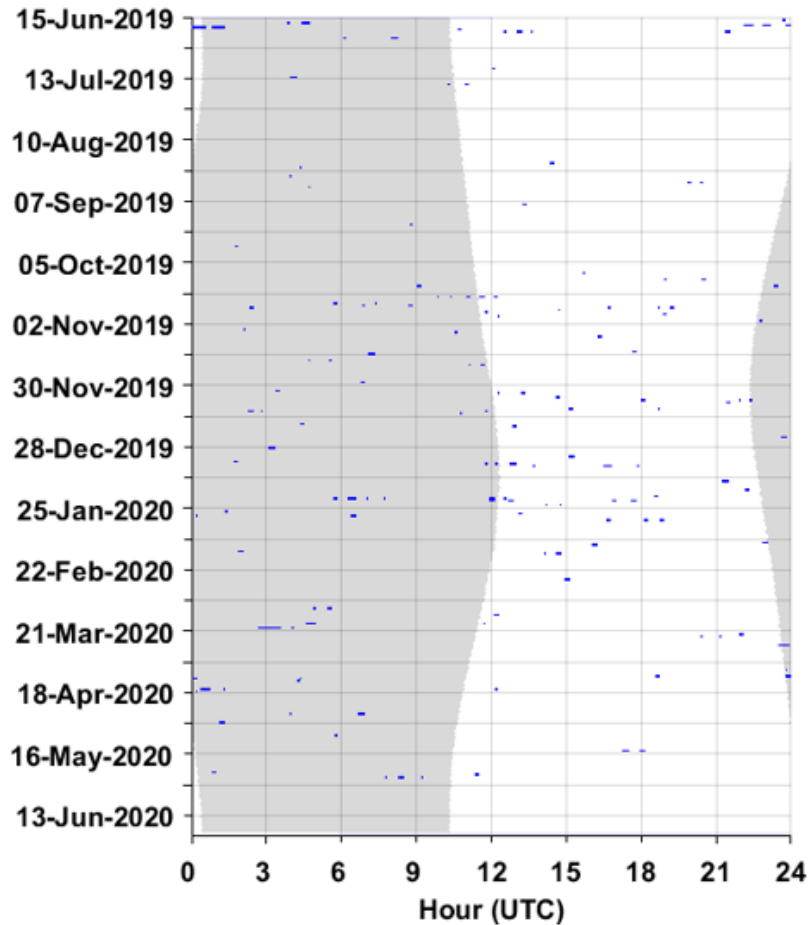
Figure 19. Kogia spp. clicks in five-minute bins from June 2019 to 2020 at JAX Site D. Effort markings are described in Figure 15.
