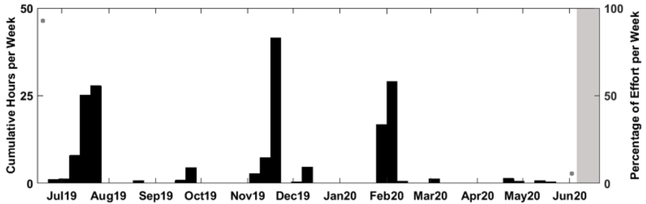
Figure 22. Weekly presence of MFA sonar less than 5 kHz from June 2019 to 2020 at JAX Site D. Effort markings are described in Figure 14.
