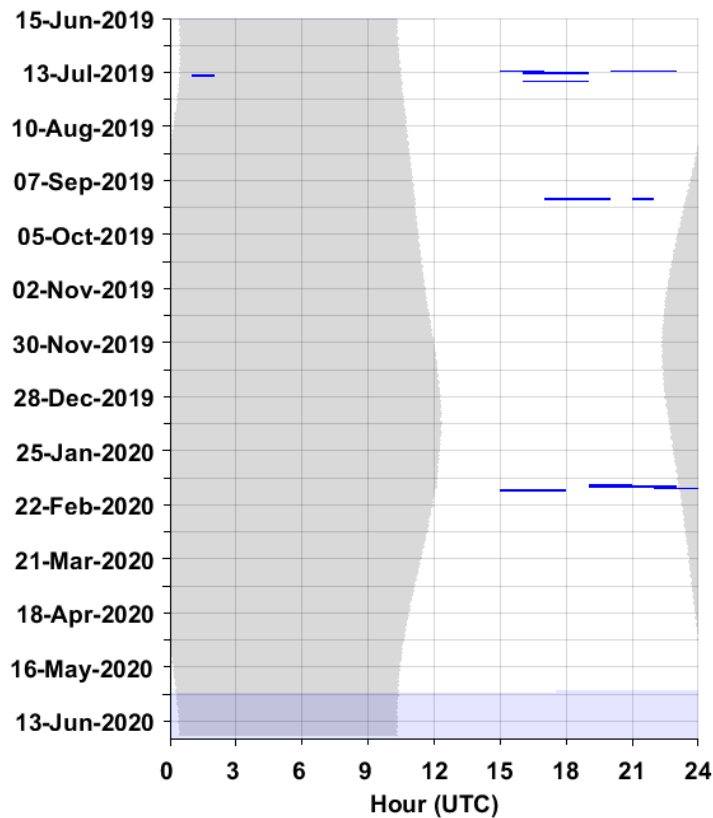
Figure 20. Weekly presence of LFA sonar from June 2019 to 2020 at JAX Site D. Effort markings are described in Figure 14.
