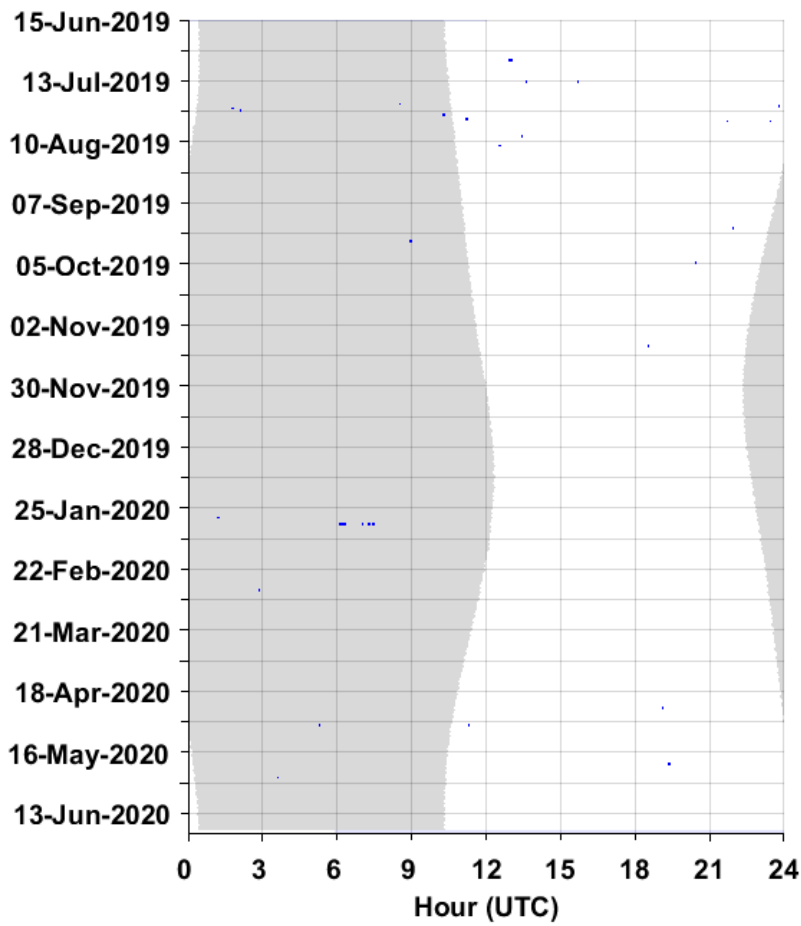
Figure 26. Explosions in five-minute bins from June 2019 to 2020 at JAX Site D. Effort markings are described in Figure 16.
