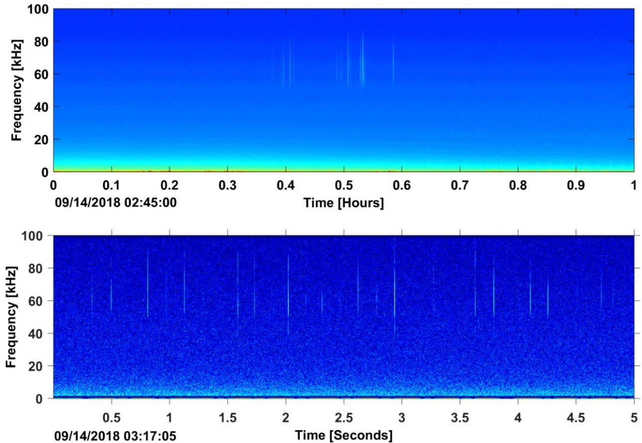
Figure 7. Sowerby's beaked whale echolocation clicks in LTSA (top) and spectrogram (bottom) recorded at JAX Site D, September 2018.
