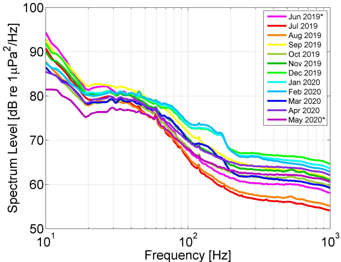
Figure 12. Monthly averages of ambient soundscape at JAX Site D from June 2019 to 2020. Legend gives color coding by month. Months with an asterisk are partial recording periods.
