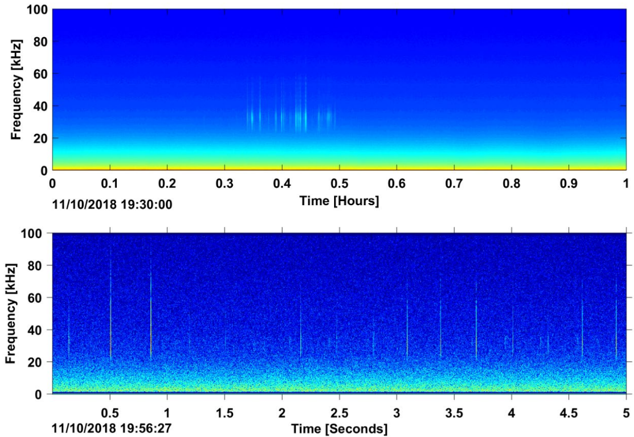
Figure 3. Blainville's beaked whale echolocation clicks in the LTSA (top) and spectrogram (bottom) recorded at JAX Site D, November 2018.
