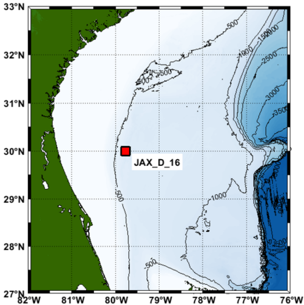
Figure 1. Location of High-Frequency Acoustic Recording Package (HARP) at JAX Site D (30° 09.28 N, 79° 46.25 W, depth 802 m) deployed in the Jacksonville Range Complex study area from June 2019 to June 2020.
