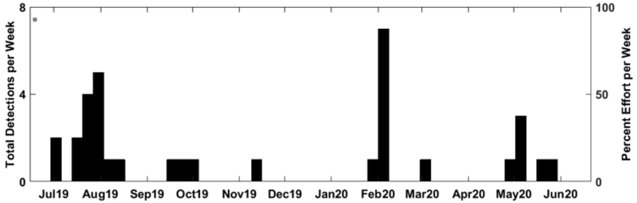
Figure 25. Weekly presence of explosions detected from June 2019 to 2020 at JAX Site D. Effort markings are described in Figure 15.
