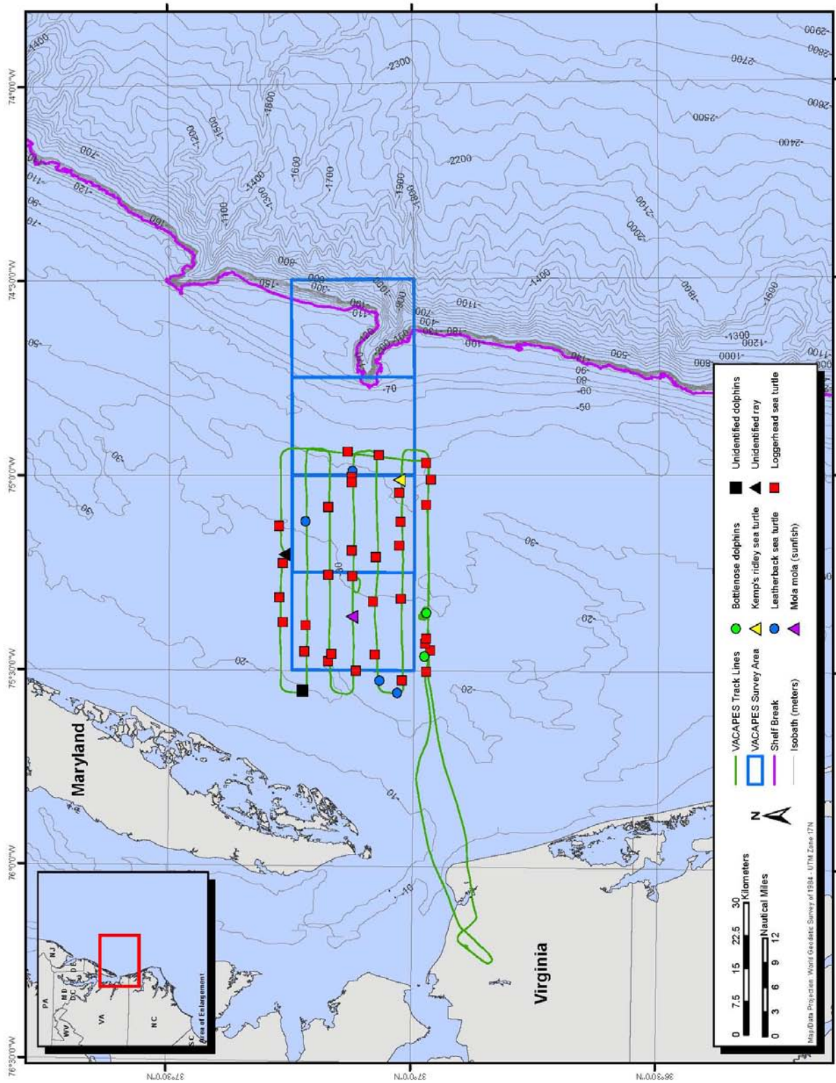
Figure 3. Location of Cetacean and Sea Turtle Sightings Seen Pre-FIREX (13 July).
