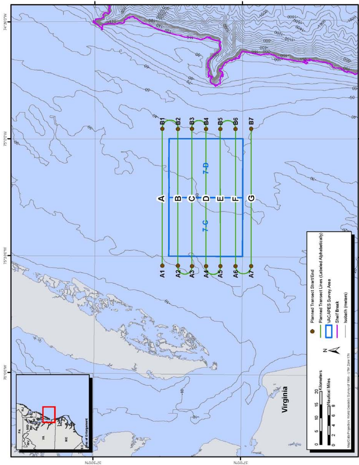
Figure 1. Predetermined Tracklines for the Survey Effort for VACAPES FIREX 2011.
